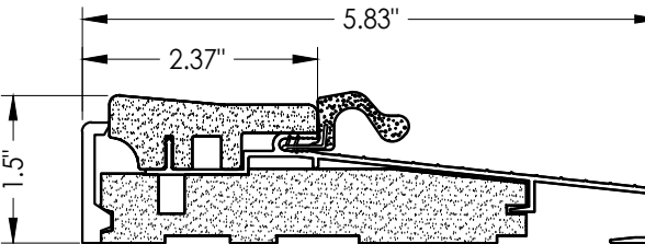
16 OUTSWING THRESHOLD
